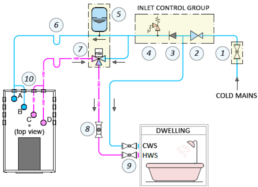
Figure 8 - Thermino 300 ePlus plumbing diagram
